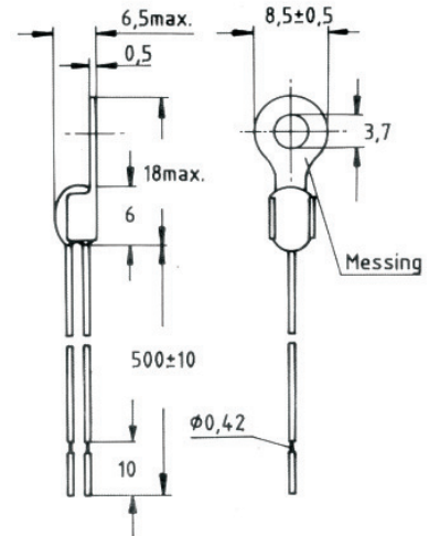
Pt-sensor in cable shoe - surface sensor
